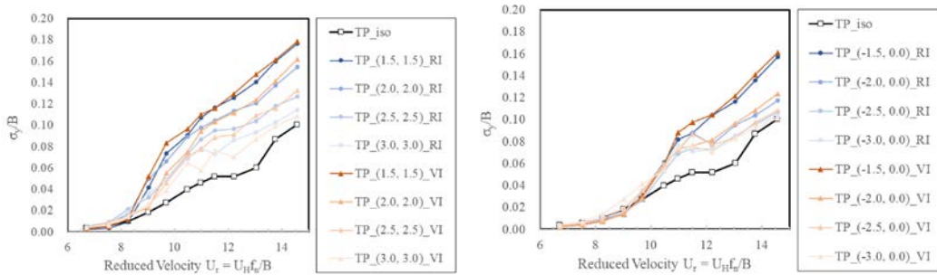
Fig. 4 TP cases for fluctuating displacement (left: oblique-upwind; right: upwind)
